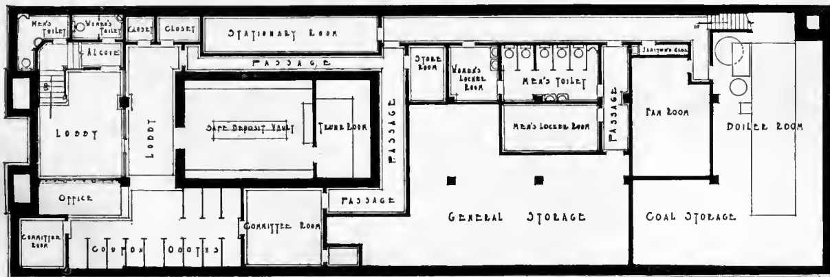
BASEMENT PLAN
